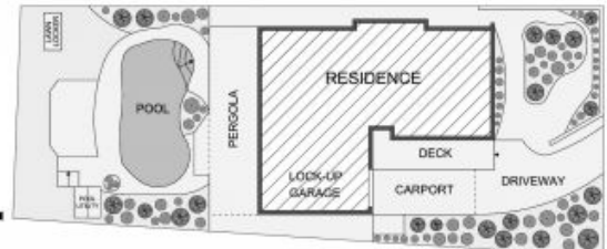
SITE PLAN
